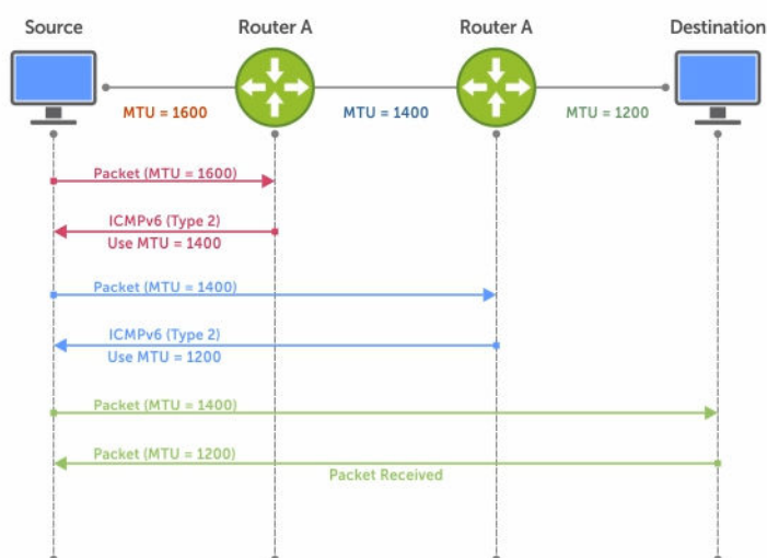
Figure 48. Path MTU Discovery Process
